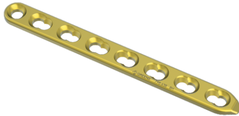
LCP PLATE 2.7 MM
